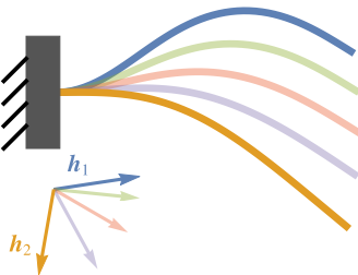
Figure 5: Controlled motion of the actuator obtained by varying the external magnetic between (h_{x1}, h_{y1}) = (13.2, 2.2) and (h_{x2}, h_{y2}) = (-1.3, -7.4) . Each shape of the actuator is the solution of the equilibrium problem (3) with \alpha and m in Fig. 4; the intermediate arrows correspond to the intermediate configurations.
