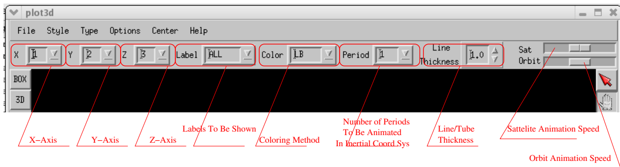
Figure 8.8: Menu-bar layout
